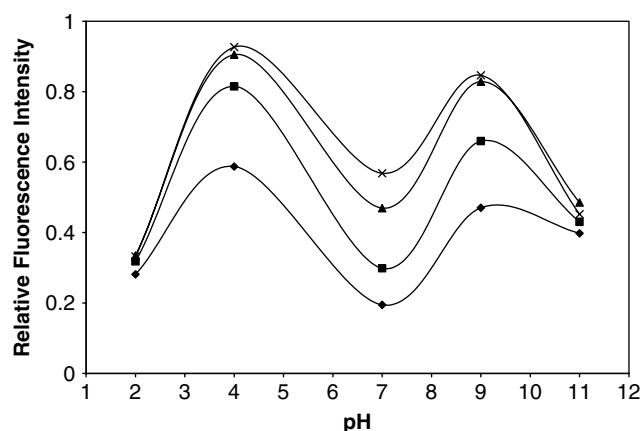
Figure 3. Effect of pH on fluorescent intensity of omeprazole degraded in methanolic solutions ( 0.345 \mu\text{g mL}^{-1} ). Exposure time to UV light 2 h (◆); 4 h (■); 6 h (▲); 8 h (×).
