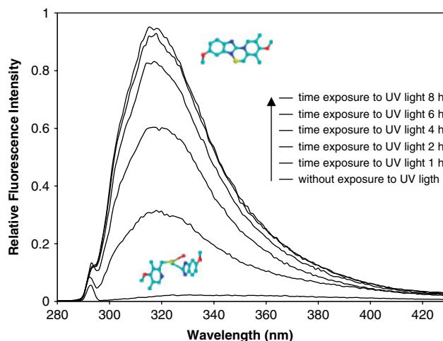
Figure 1. Fluorescent spectra of omeprazole degradation product produced by exposing the drug to direct ultraviolet light during different periods of time.
